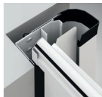
Circumferential gasket (double-lip)
